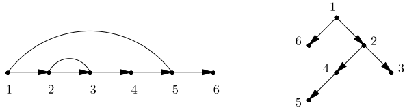
Fig. 1 A nested word and its tree translation
